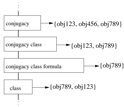
Fig. 6. Invalidation Index: an adaptive inverted index containing both words and phrases, used for determining which text objects are likely to need to be re-analyzed for linking after concept definition updates have occurred to the corpus. The structure is a chained hash, with words and phrases as hash keys, and an object identifier list for each. In the above example, if a definition for “conjugacy class formula” were added to the corpus, only object 789 would need to be invalidated.
