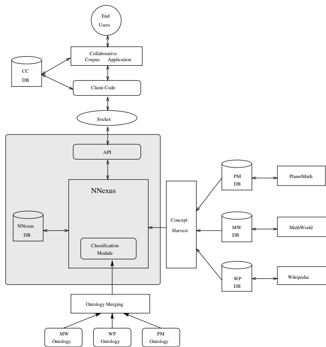
Fig. 7. NNexus System Architecture (in an example deployment): The shaded region denotes NNexus proper. The classification module provides classification-invariant link steering between multiple ontologies.
