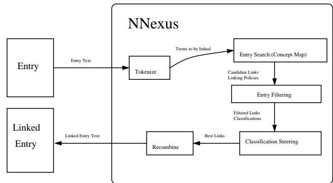
Fig. 2. Linking Diagram: When an entry is linked through NNexus the candidate links are found in the concept map. These candidates are then compared against the linking policies and sent through the classification module. The top candidate links are then recombined into the original text and returned to the user.
