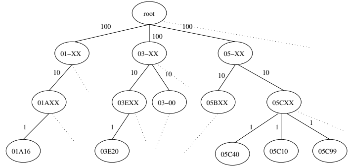
Fig. 5. Example Classification Tree: This is the MSC subject classification represented as an OWL formatted file and as a weighted graph. The weights are assigned with base 10.
