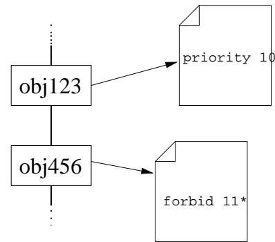
Fig. 4. The linking policy table stores a text chunk for each entry, containing optional user-supplied link-steering directives.
