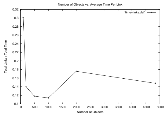
Fig. 11. Scalability study: time-per-link for progressively larger corpora, showing clearly that the automatic linking process is sub-linear in time complexity.
