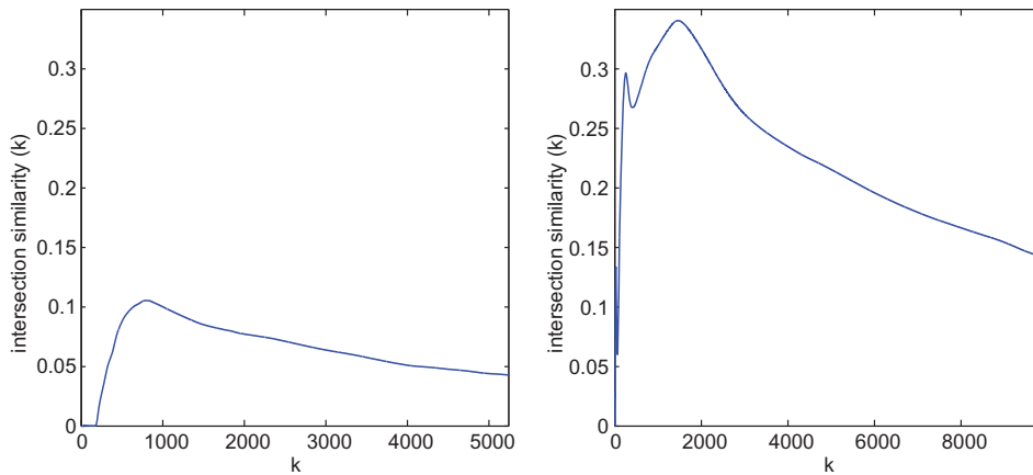
FIG. 3. The intersection distance values ( isim_k ) of the ca-GrQc (left) and the ca-HepTh (right) collaboration networks.
