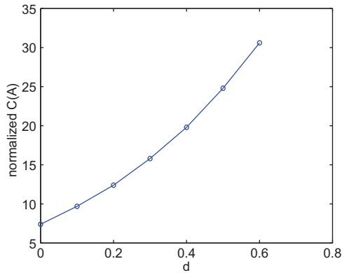
FIG. 1. Plot of the total network communicability C(A) for small-world graphs with increasing probability d of a shortcut. The computed values were averaged over 20 instances.
