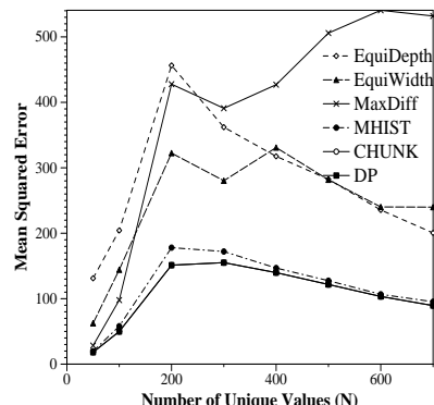
Figure 6: Effect of Data Size ( N ) on Error (D1 data set)
