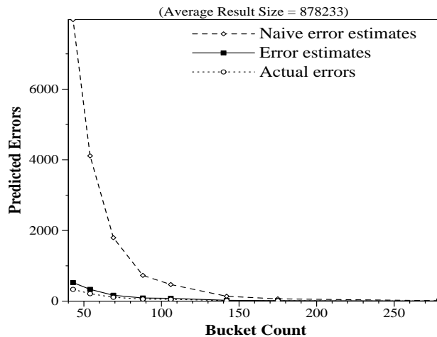
Figure 8: Quality Guarantees: Range Predicates
