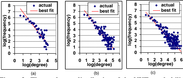
Figure 3: The outdegree distribution of the NYT reachability graph for Task 1 when (a) MaxResults = 10 , (b) MaxResults = 50 , and (c) MaxResults = 200 .
