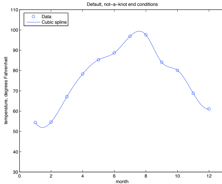
Figure 4.16: Cubic polynomial spline interpolant, using not-a-knot end conditions, for average high temperature data given in Example 4.5.3
