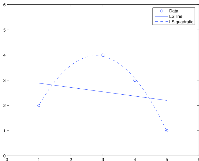
Figure 4.20: Linear and quadratic polynomial least squares fit of data given in Example 4.5.12
