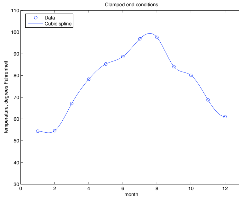
Figure 4.17: Cubic polynomial spline interpolant, using clamped end conditions, for average high temperature data given in Example 4.5.3
