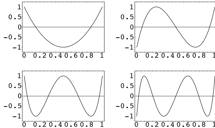
Figure 4.10: The shifted Chebyshev polynomials T_2(\bar{x}) top left; T_3(\bar{x}) top right; T_4(\bar{x}) bottom left, T_5(\bar{x}) bottom right.
