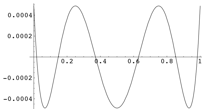
Figure 4.7: Plot of the polynomial \omega_{N+1}(x) for x \in [0, 1] when a = 0 , b = 1 and N = 5 with Chebyshev nodes.
