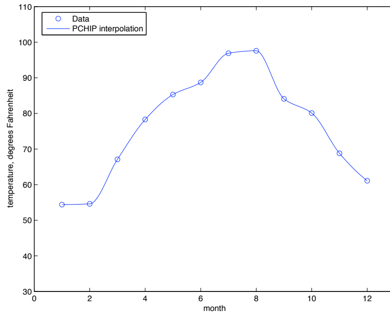
Figure 4.18: Piecewise cubic Hermite interpolating polynomial, for average high temperature data given in Example 4.5.3
