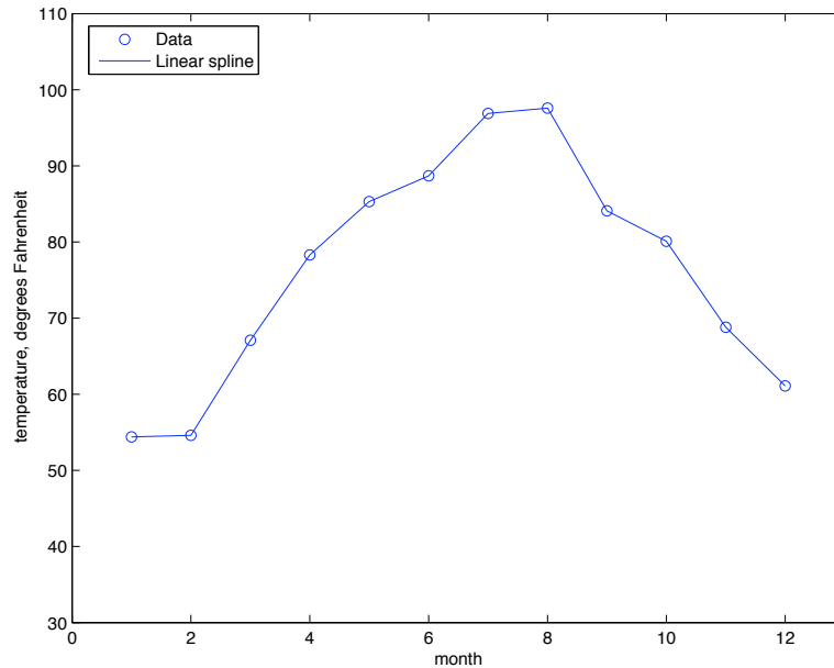
Figure 4.15: Linear polynomial spline interpolant for average high temperature data given in Example 4.5.3
