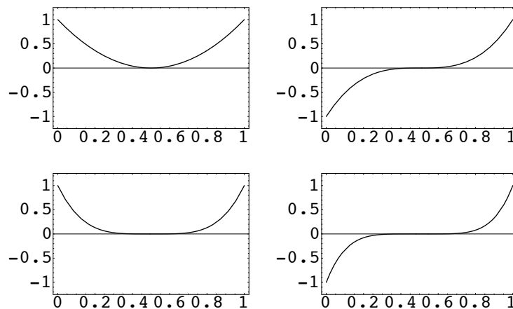
Figure 4.11: The powers \bar{x}^2 top left; \bar{x}^3 top right; \bar{x}^4 bottom left, \bar{x}^5 bottom right.
