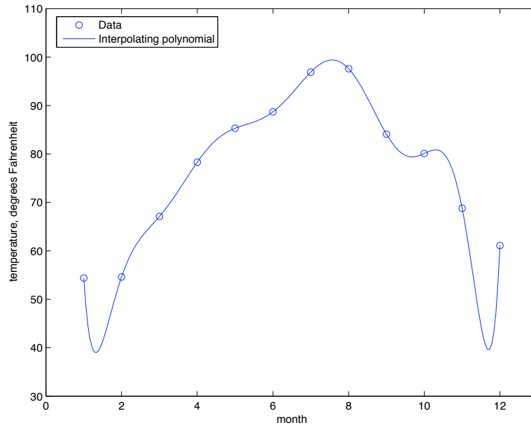
Figure 4.13: Interpolating polynomial from Example 4.5.3
