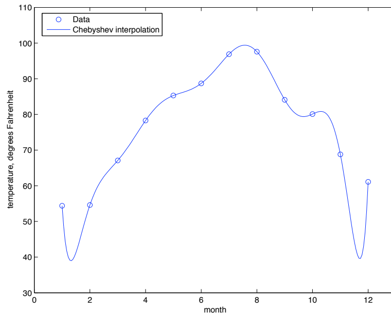
Figure 4.19: Interpolating polynomial or average high temperature data given in Example 4.5.3 using the Chebyshev form.
