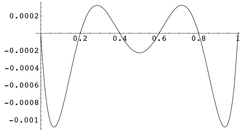
Figure 4.5: Plot of the polynomial \omega_{N+1}(x) for x \in [0, 1] when a = 0, b = 1, N = 5 with equally spaced nodes.
