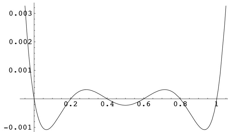
Figure 4.6: Plot of the polynomial \omega_{N+1}(x) for x \in [-0.05, +1.05] when a = 0, b = 1, and N = 5 with equally spaced nodes.
