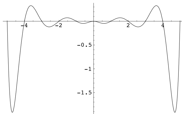
Figure 4.8: The error in interpolating f(x) = \frac{1}{1+x^2} by a polynomial on the interval [-5, +5] for 11 equally spaced nodes ( N = 10 ).
