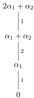
Non-negative weights of standard representation
