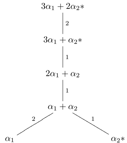
Positive roots (Long roots marked with a *)
